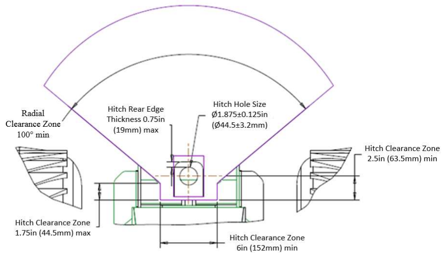
Figure A-2 Requirements of the Hitch Design
