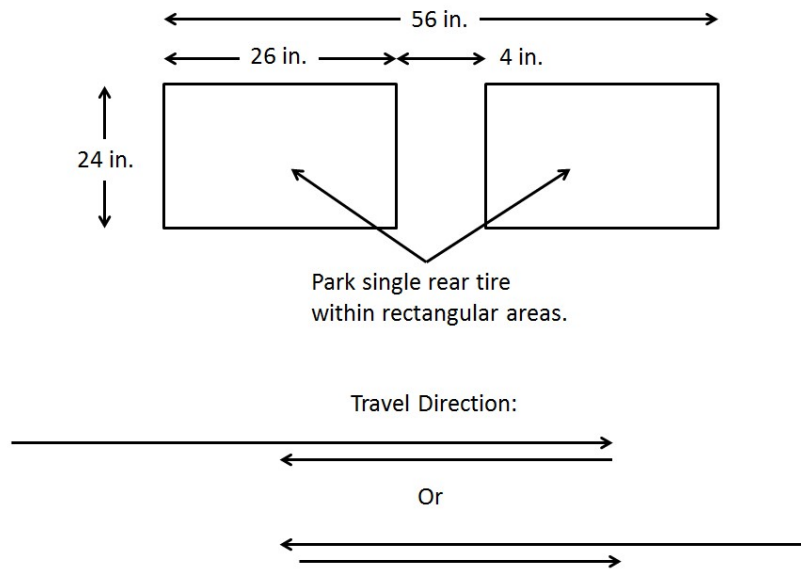
Figure A-13 Controllability Test Layout
