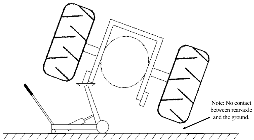
Figure A-6 Wheelie Bar Test
