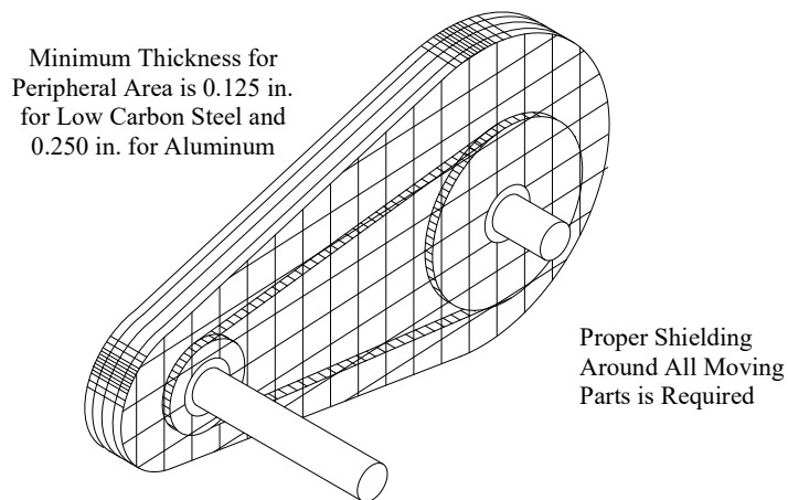
Figure A-3 Example of Proper Shielding for Moving Parts
