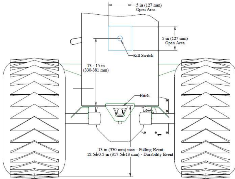
Figure A-4 Hitch and Kill Switch Specifications
