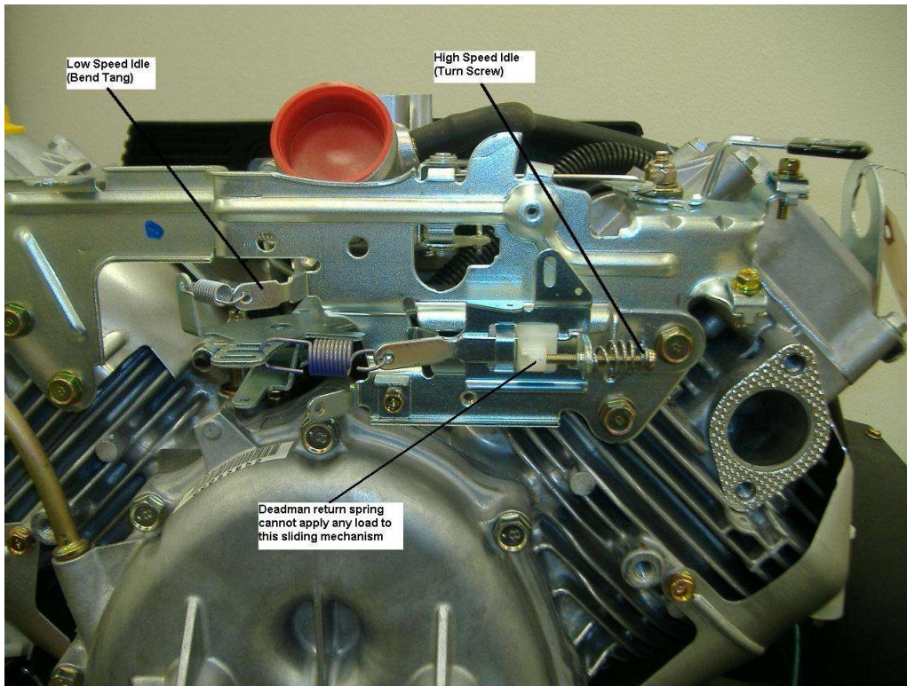
Figure A-7 31-hp Engine Throttle Cable Mechanism
